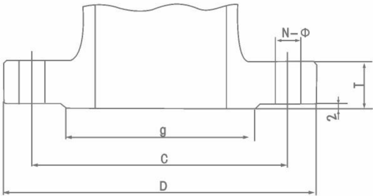
Class 150 / 300Lb (RF)Steel
