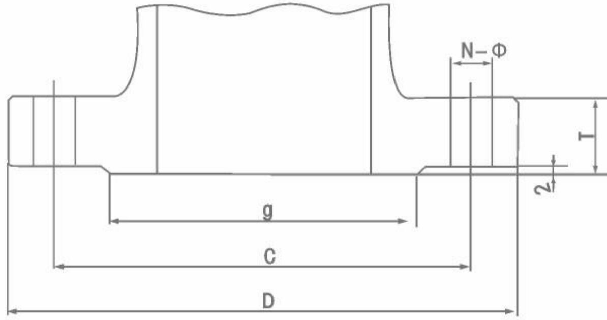
Class 600Lb (RF)Steel
